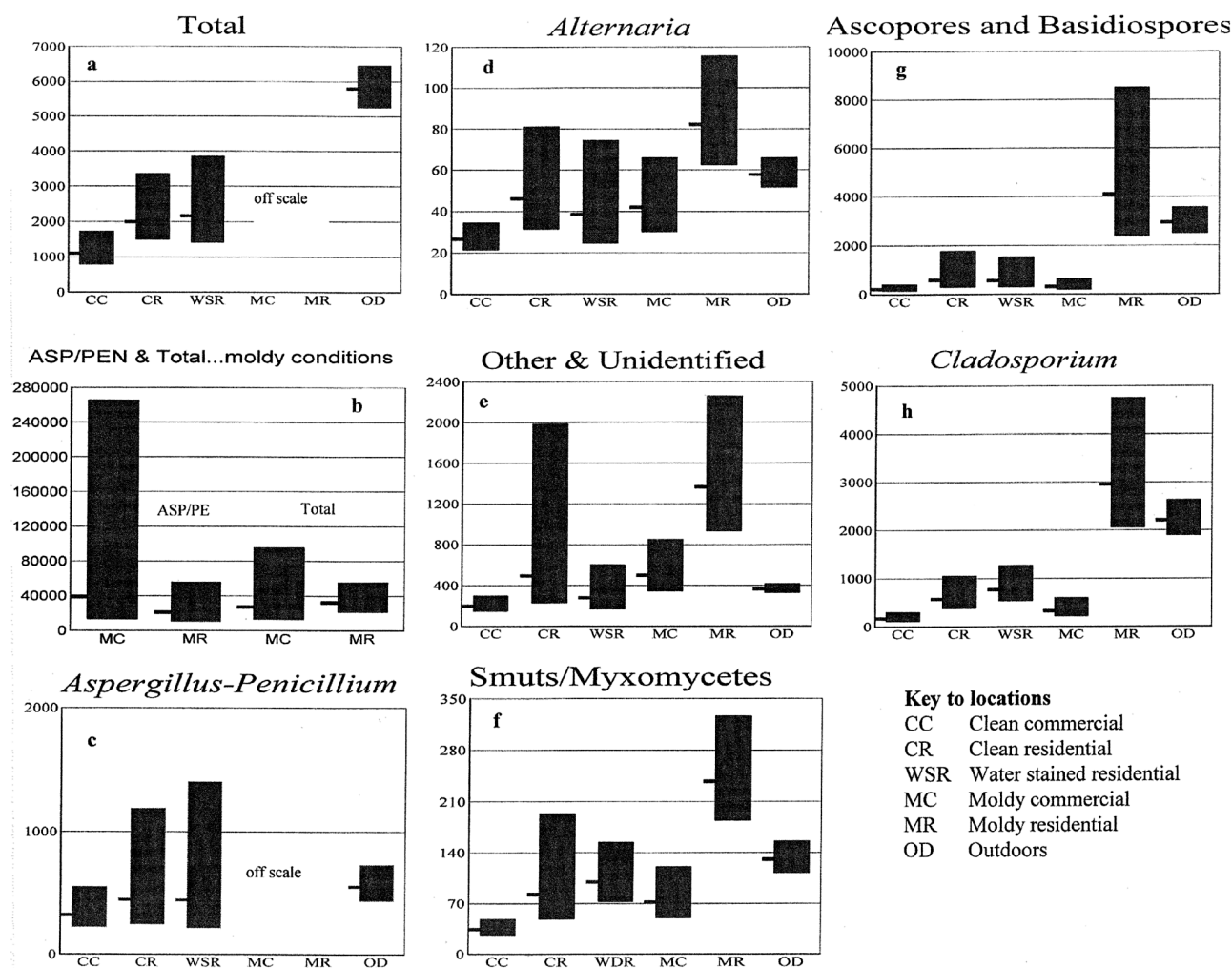
FIGURE 1. Maximum likelihood estimate of mean spore count/m 3 of air (small horizontal bar) and 90% confidence limits for the mean (large vertical bar) for seven fungal groups and six location types. Note that for Aspergillus/Penicillium and Total, the data for moldy buildings is separated in (b) to preserve scale in (a) and (c).
